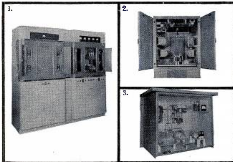
1. A Collins phasor (left) alongside Collins transmitter. Phasor can be furnished to match most makes of transmitters. 2. Antenna tuning unit. 3. Interior view of 5 kw phasor, illustrates compactness and convenience of Collins design.
